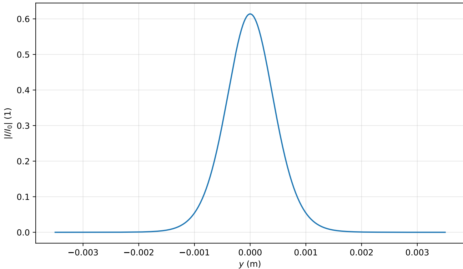
Intensity profile I(x=0, y, z=2.786)/I_0 , P_{in}=0.5P_{cr} , artificial time
